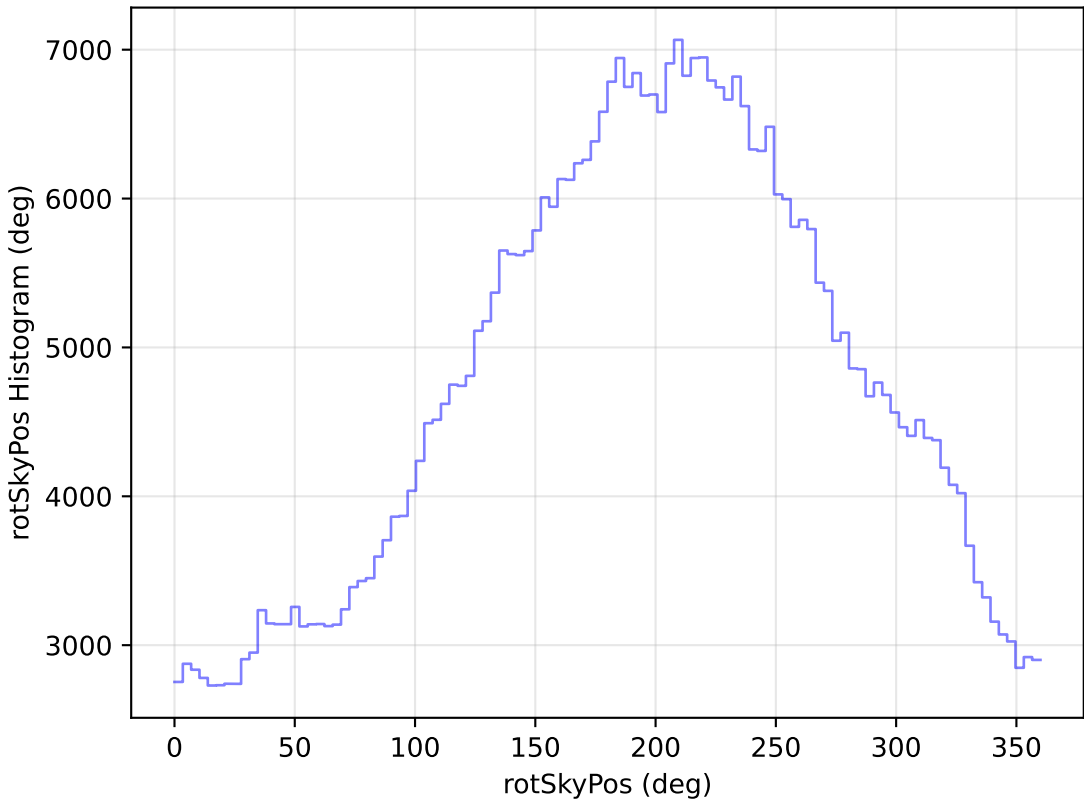
ddf_loaded_fl2_v3.4_10yrs WFD r band: rotSkyPos Histogram
