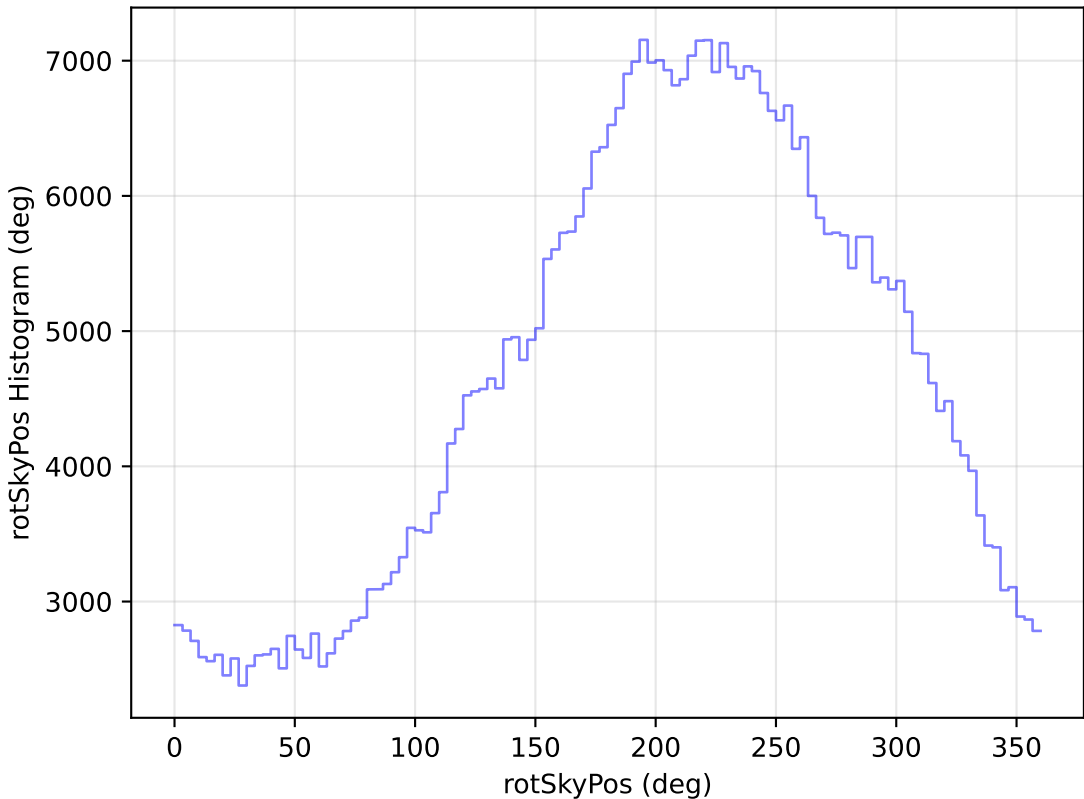
ddf_loaded_fl2_v3.4_10yrs WFD i band: rotSkyPos Histogram
