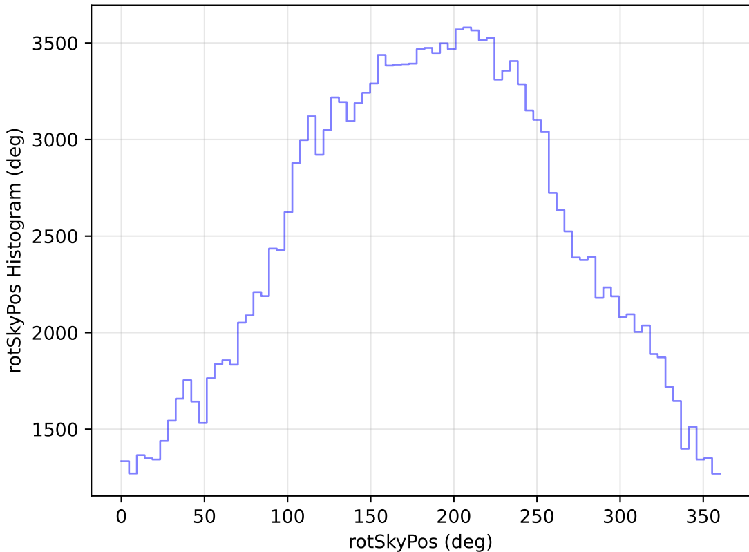
ddf_loaded_fl2_v3.4_10yrs WFD g band: rotSkyPos Histogram
