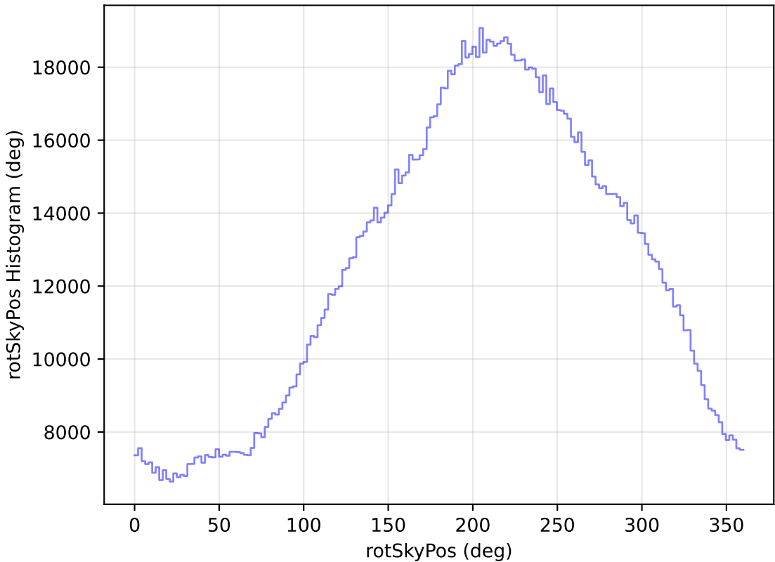
ddf_loaded_fl2_v3.4_10yrs WFD all bands: rotSkyPos Histogram
