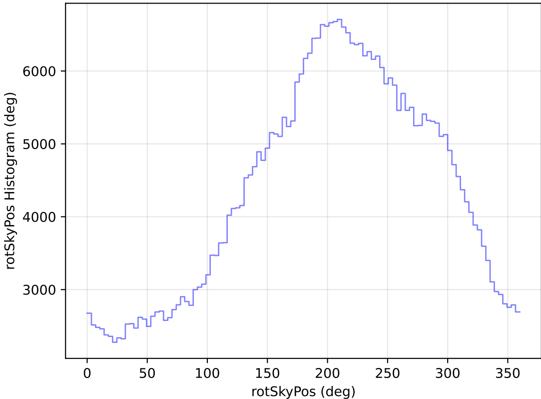
ddf_loaded_fl2_v3.4_10yrs All sky z band: rotSkyPos Histogram
