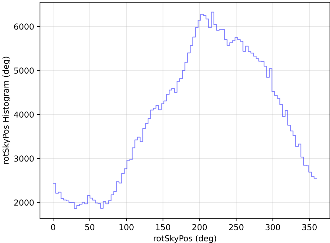
ddf_loaded_fl2_v3.4_10yrs All sky y band: rotSkyPos Histogram
