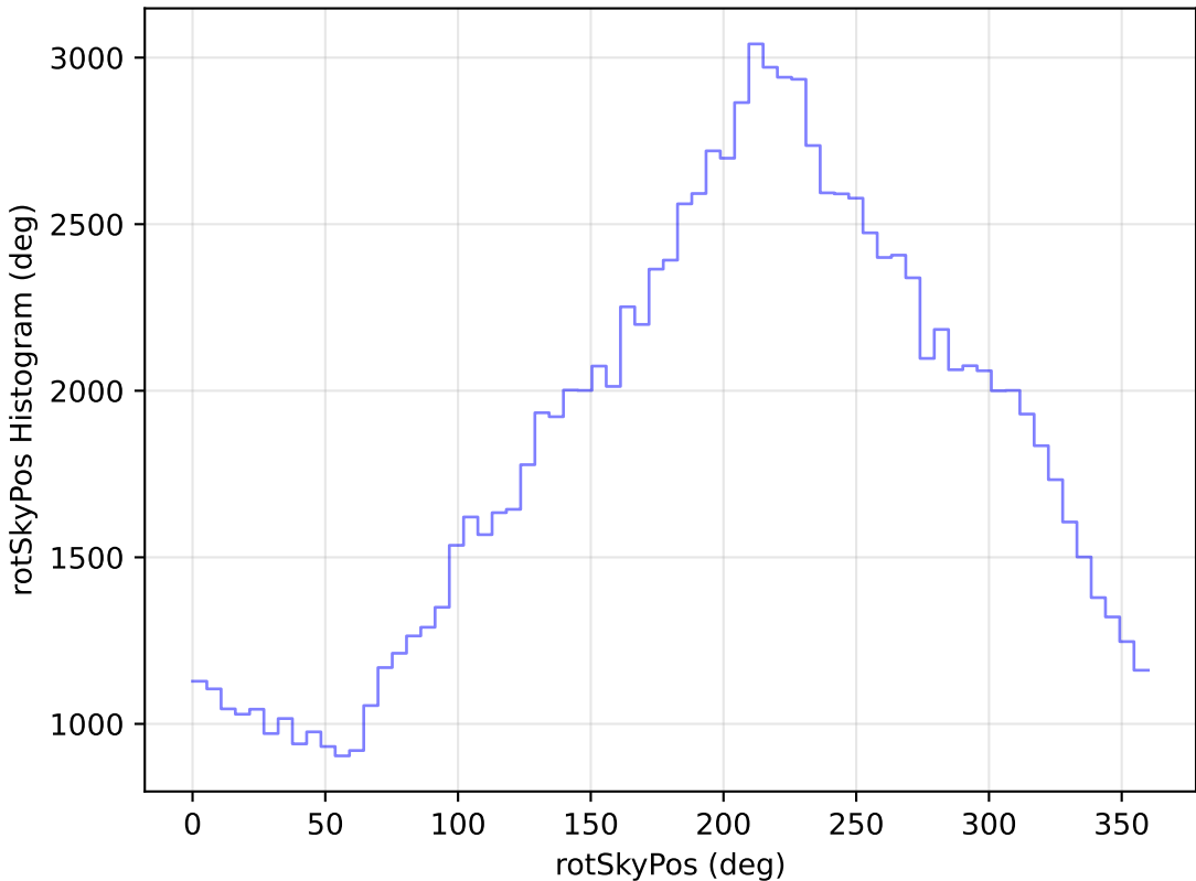
ddf_loaded_fl2_v3.4_10yrs All sky u band: rotSkyPos Histogram
