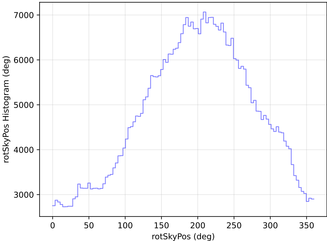
ddf_loaded_fl2_v3.4_10yrs All sky r band: rotSkyPos Histogram
