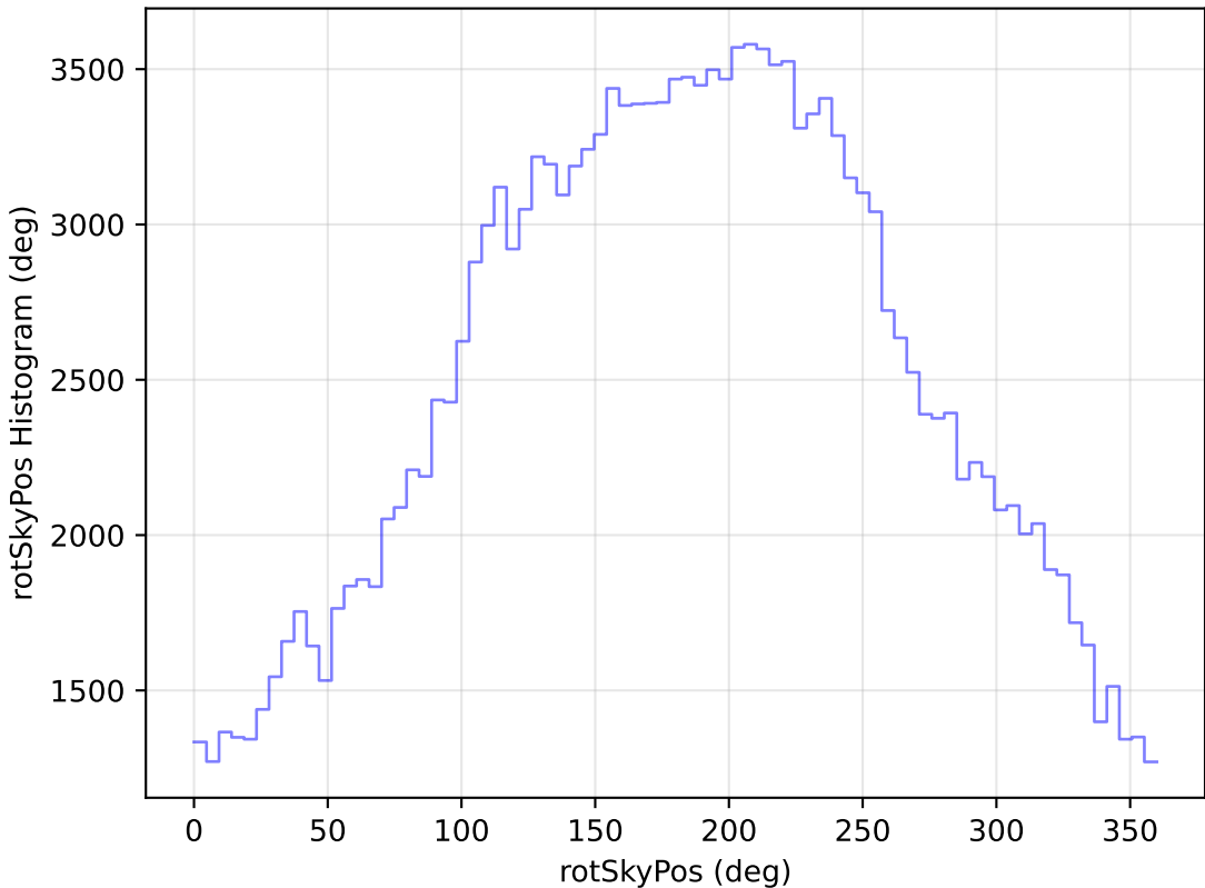
ddf_loaded_fl2_v3.4_10yrs All sky g band: rotSkyPos Histogram
