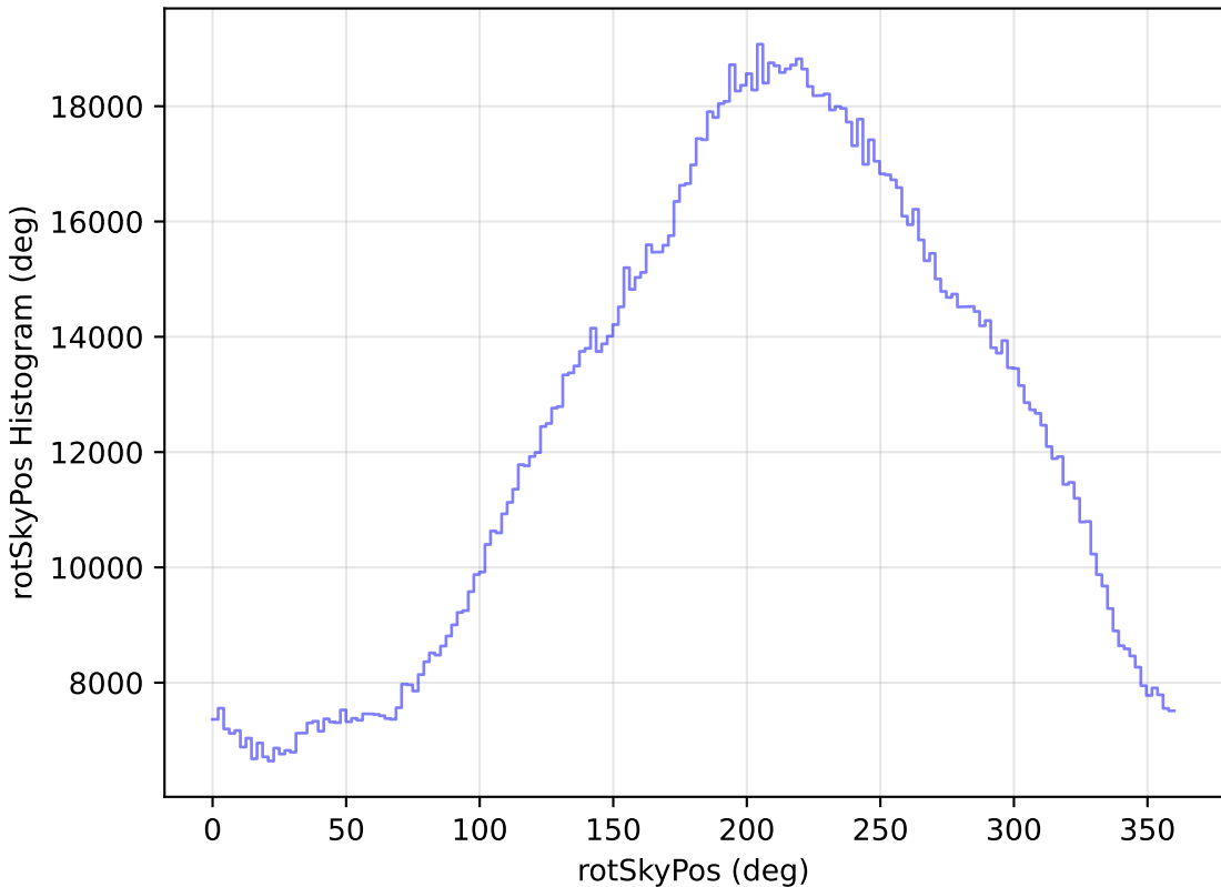
ddf_loaded_fl2_v3.4_10yrs All sky all bands: rotSkyPos Histogram
