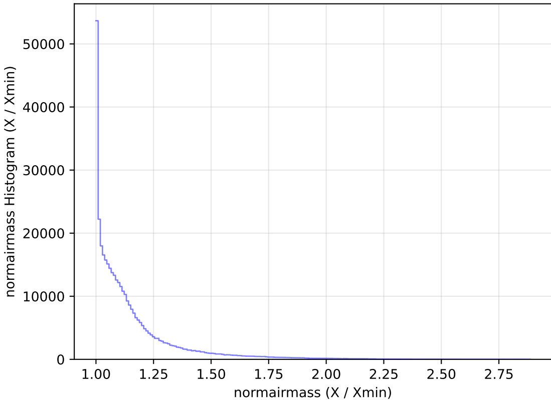
ddf_loaded_fl2_v3.4_10yrs WFD y band: normairmass Histogram
