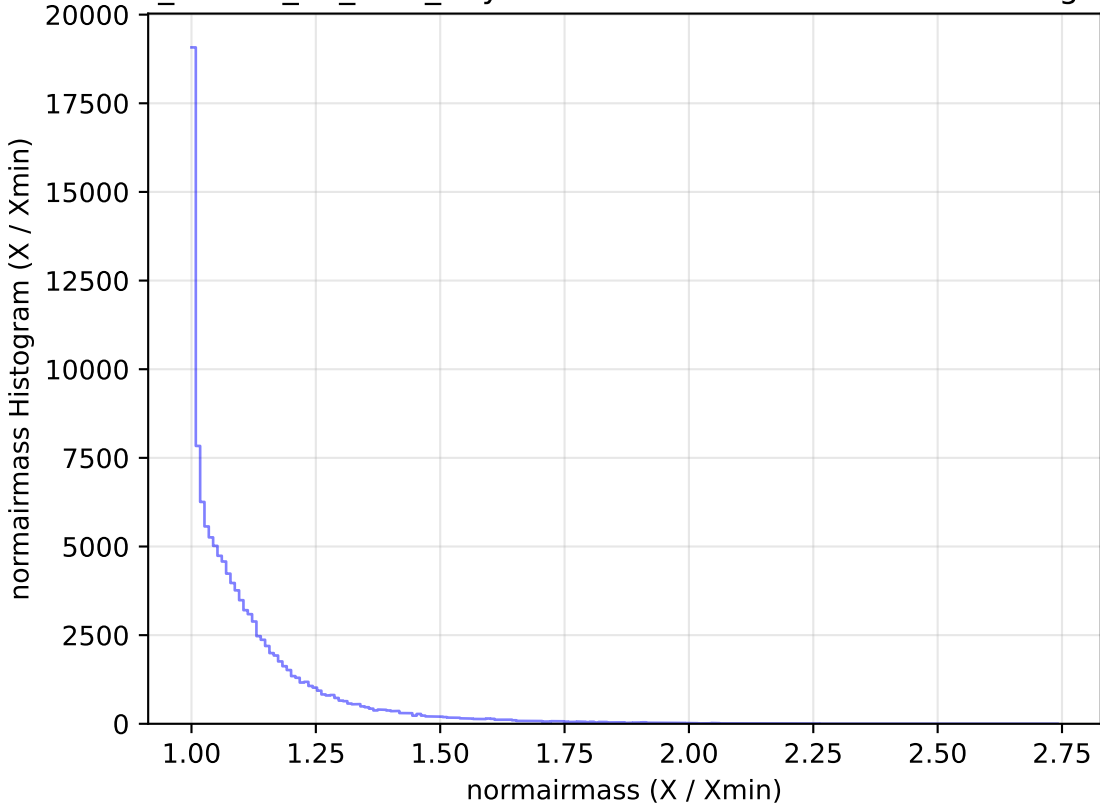
ddf_loaded_fl2_v3.4_10yrs WFD u band: normairmass Histogram
