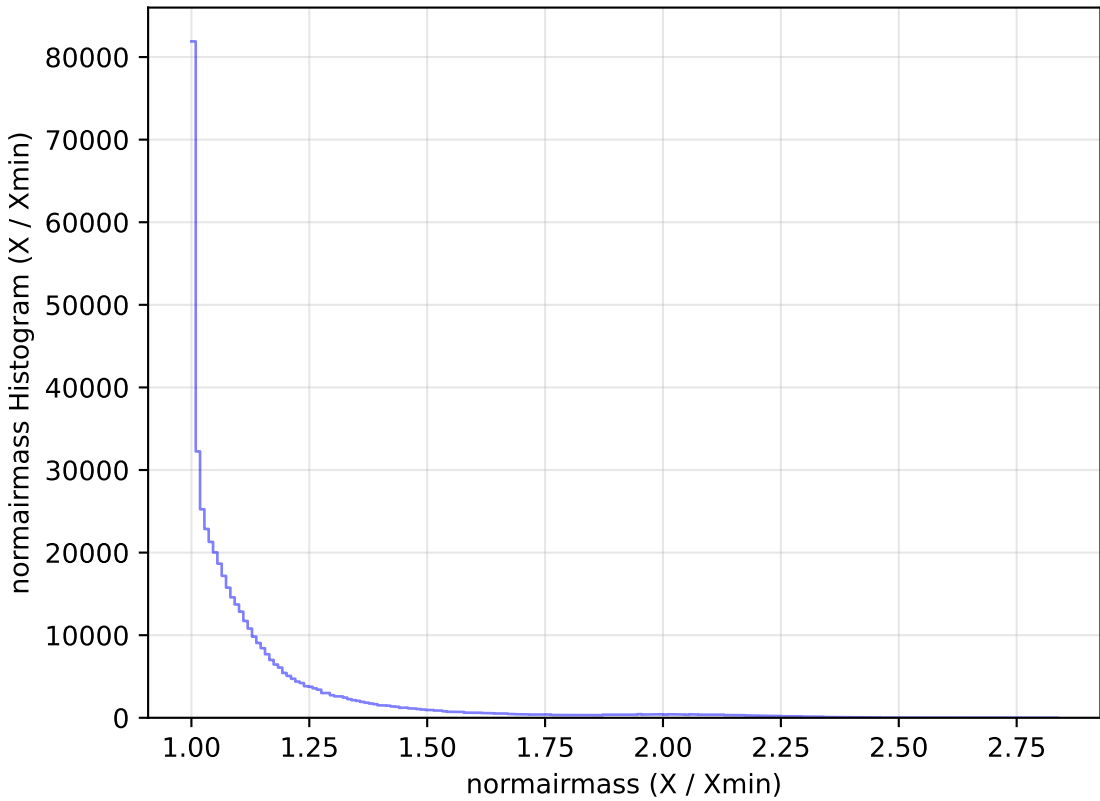
ddf_loaded_fl2_v3.4_10yrs WFD r band: normairmass Histogram
