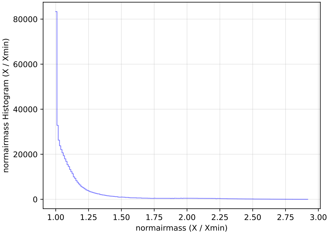
ddf_loaded_fl2_v3.4_10yrs WFD i band: normairmass Histogram
