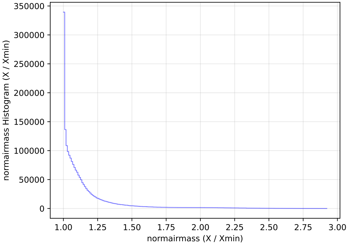
ddf_loaded_fl2_v3.4_10yrs WFD all bands: normairmass Histogram
