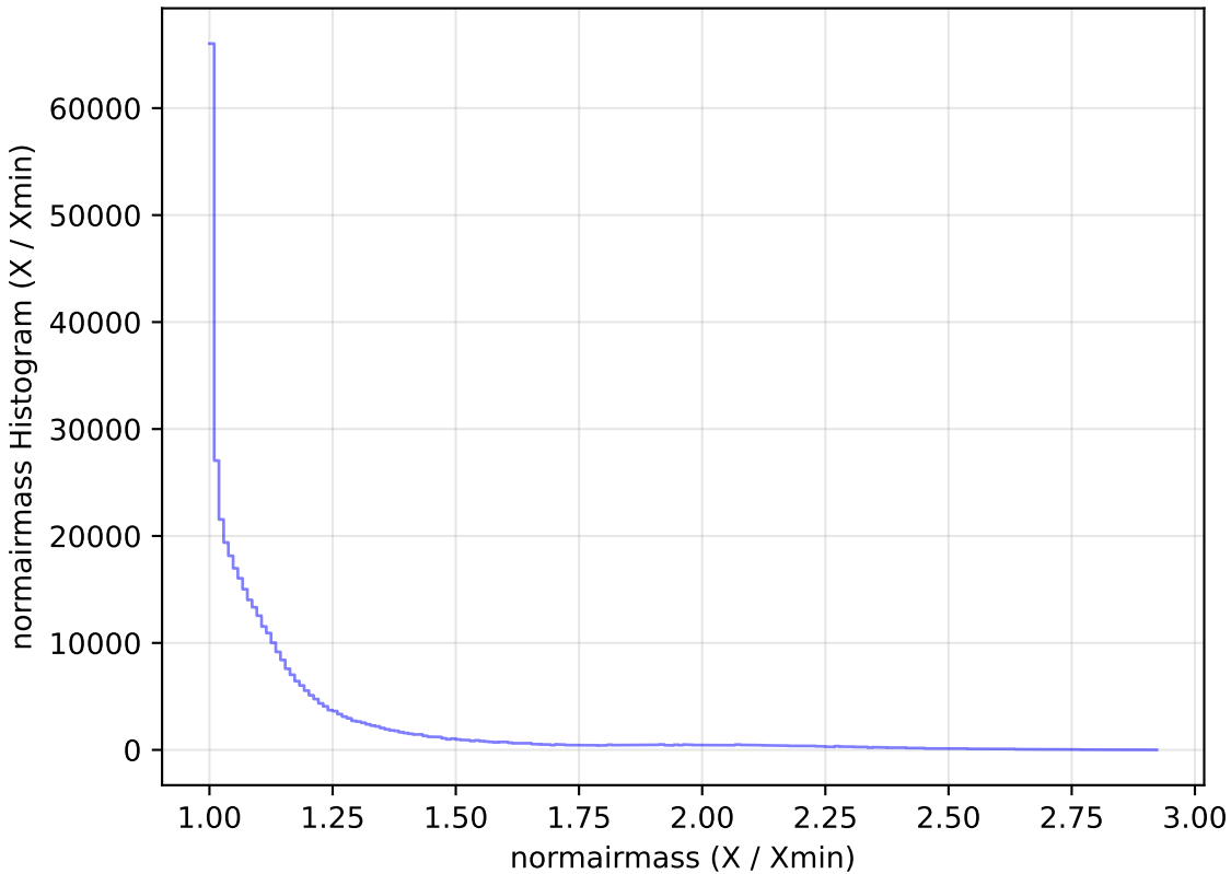
ddf_loaded_fl2_v3.4_10yrs All sky z band: normairmass Histogram
