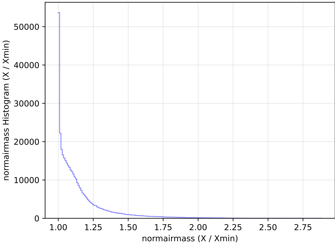
ddf_loaded_fl2_v3.4_10yrs All sky y band: normairmass Histogram
