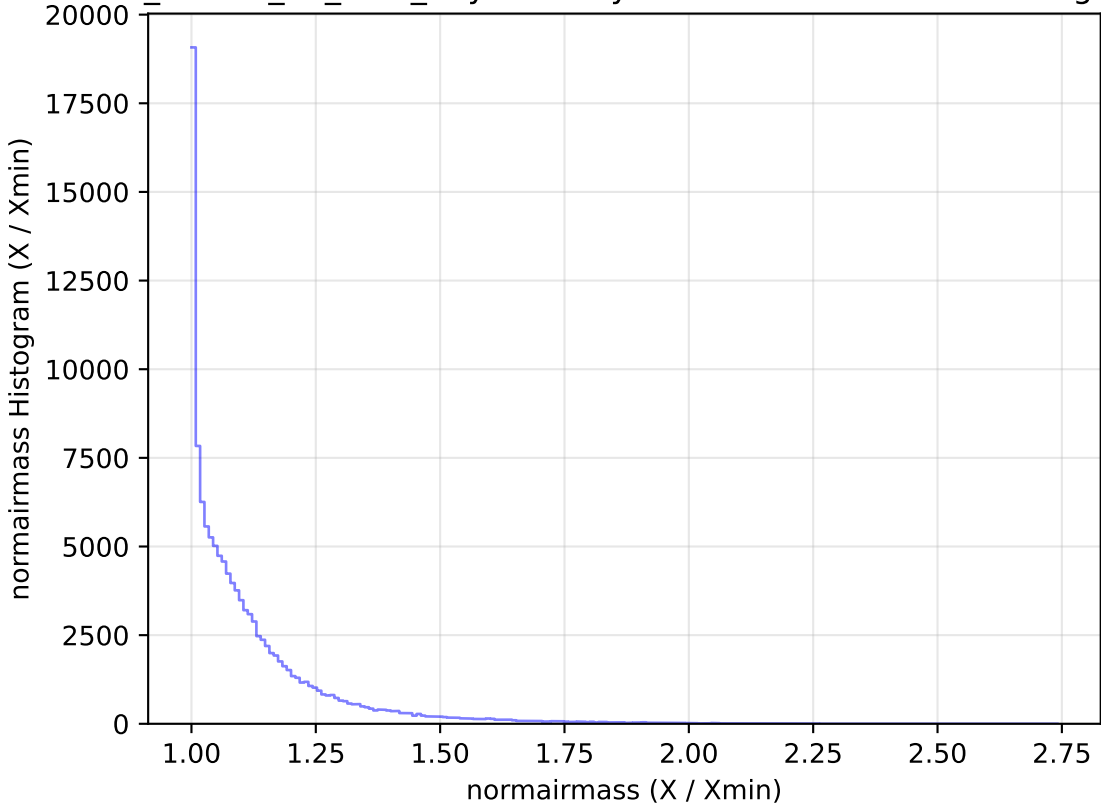
ddf_loaded_fl2_v3.4_10yrs All sky u band: normairmass Histogram
