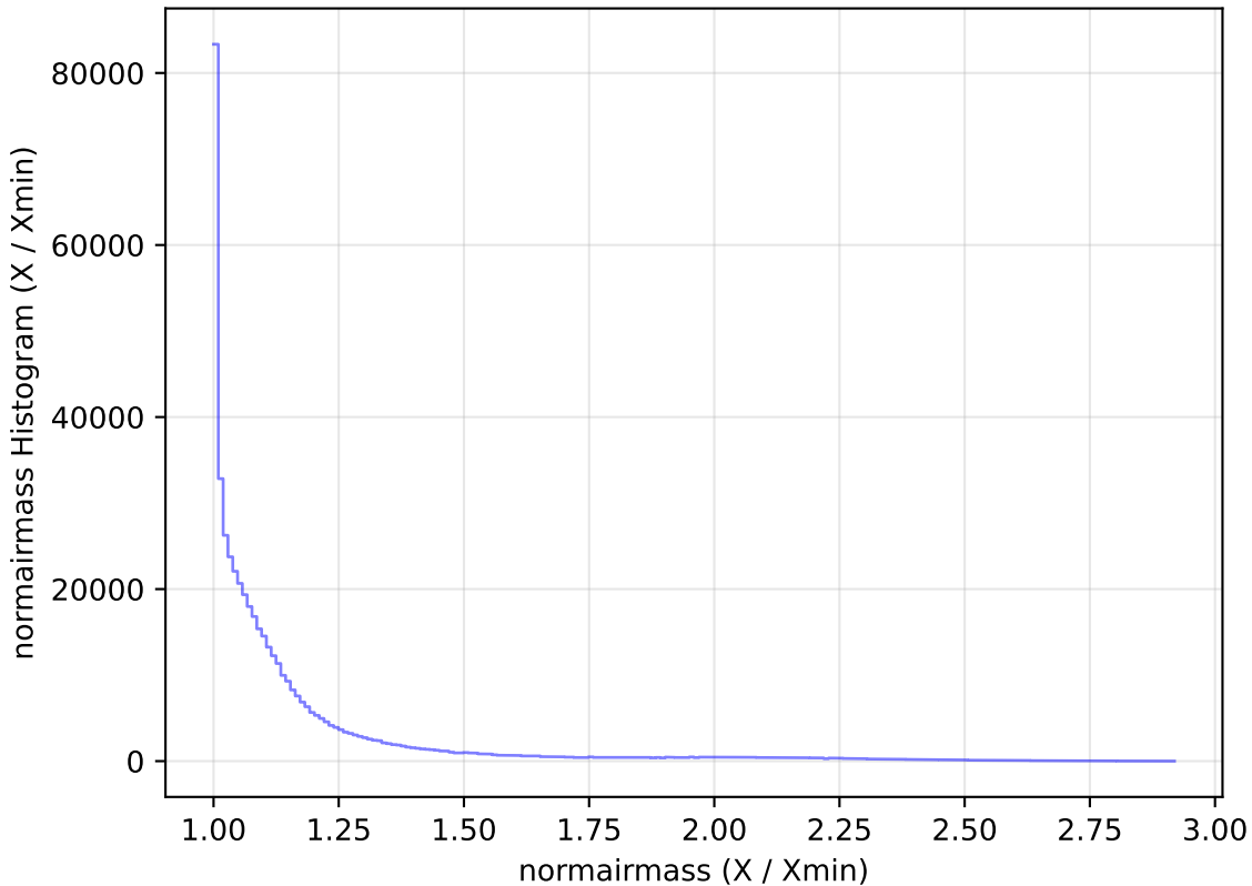
ddf_loaded_fl2_v3.4_10yrs All sky i band: normairmass Histogram
