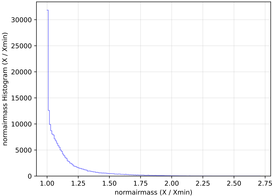
ddf_loaded_fl2_v3.4_10yrs All sky g band: normairmass Histogram
