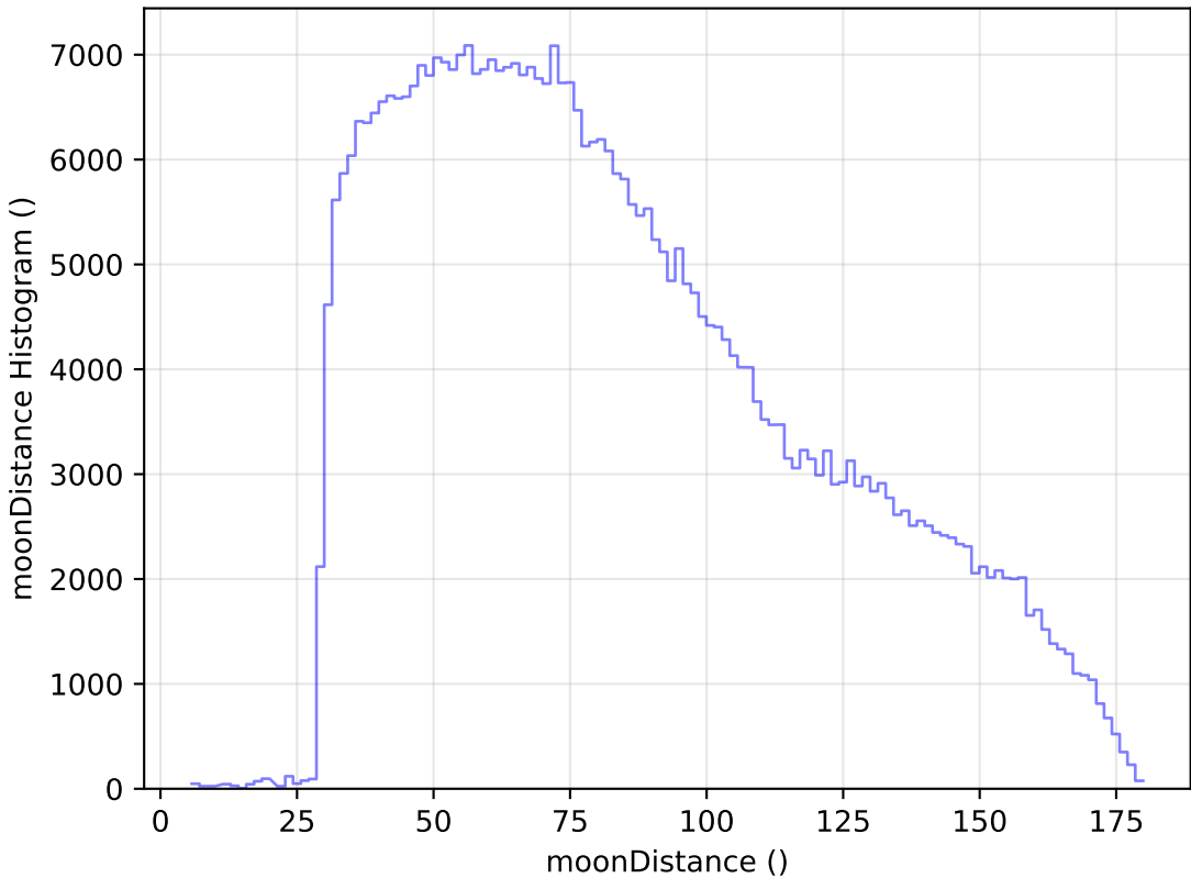
ddf_loaded_fl2_v3.4_10yrs WFD z band: moonDistance Histogram
