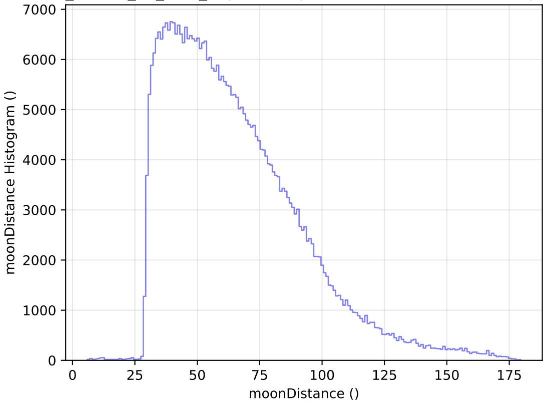
ddf_loaded_fl2_v3.4_10yrs WFD y band: moonDistance Histogram
