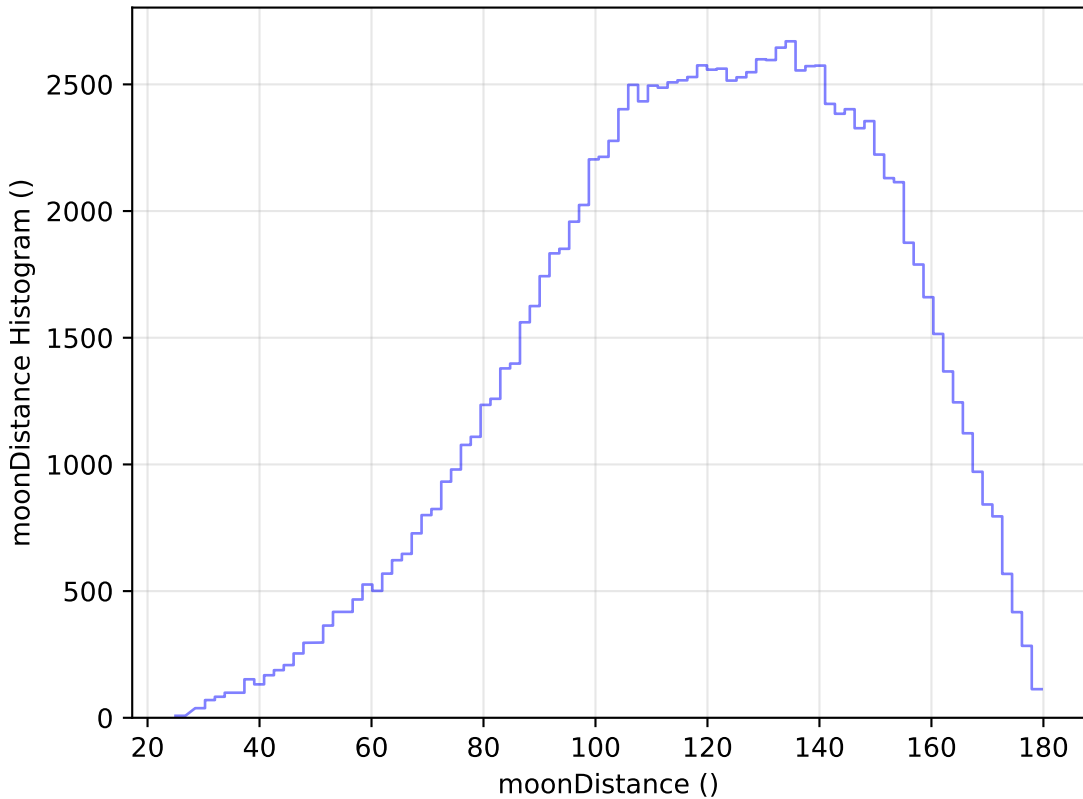
ddf_loaded_fl2_v3.4_10yrs WFD u band: moonDistance Histogram
