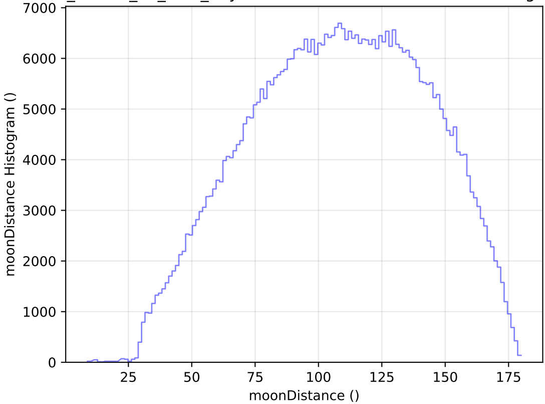
ddf_loaded_fl2_v3.4_10yrs WFD r band: moonDistance Histogram
