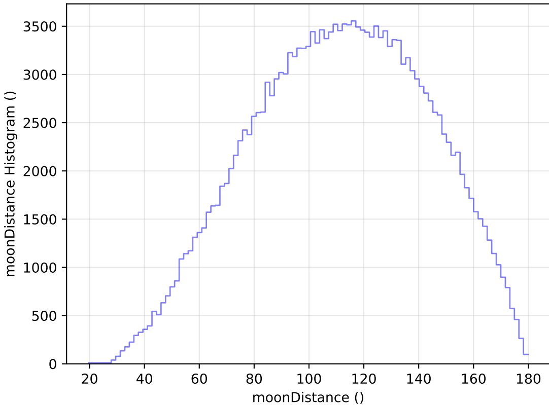
ddf_loaded_fl2_v3.4_10yrs WFD g band: moonDistance Histogram
