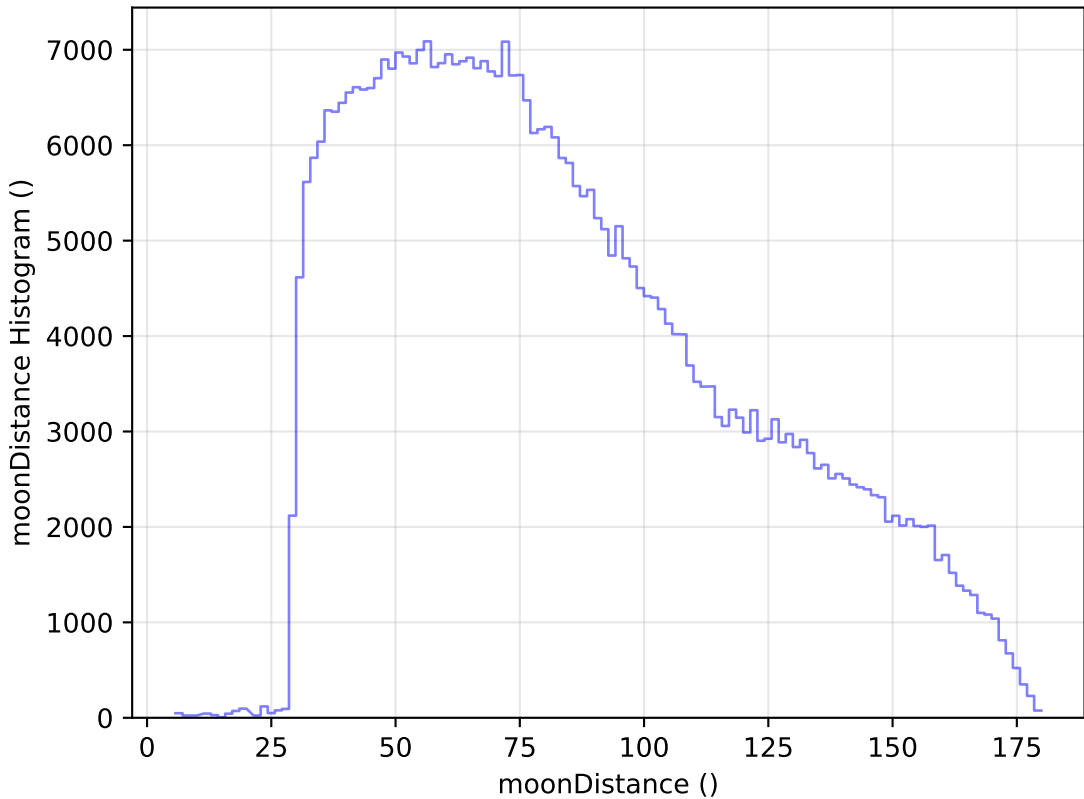
ddf_loaded_fl2_v3.4_10yrs All sky z band: moonDistance Histogram
