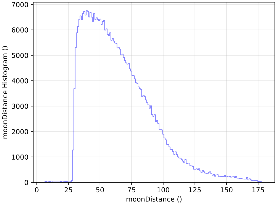
ddf_loaded_fl2_v3.4_10yrs All sky y band: moonDistance Histogram
