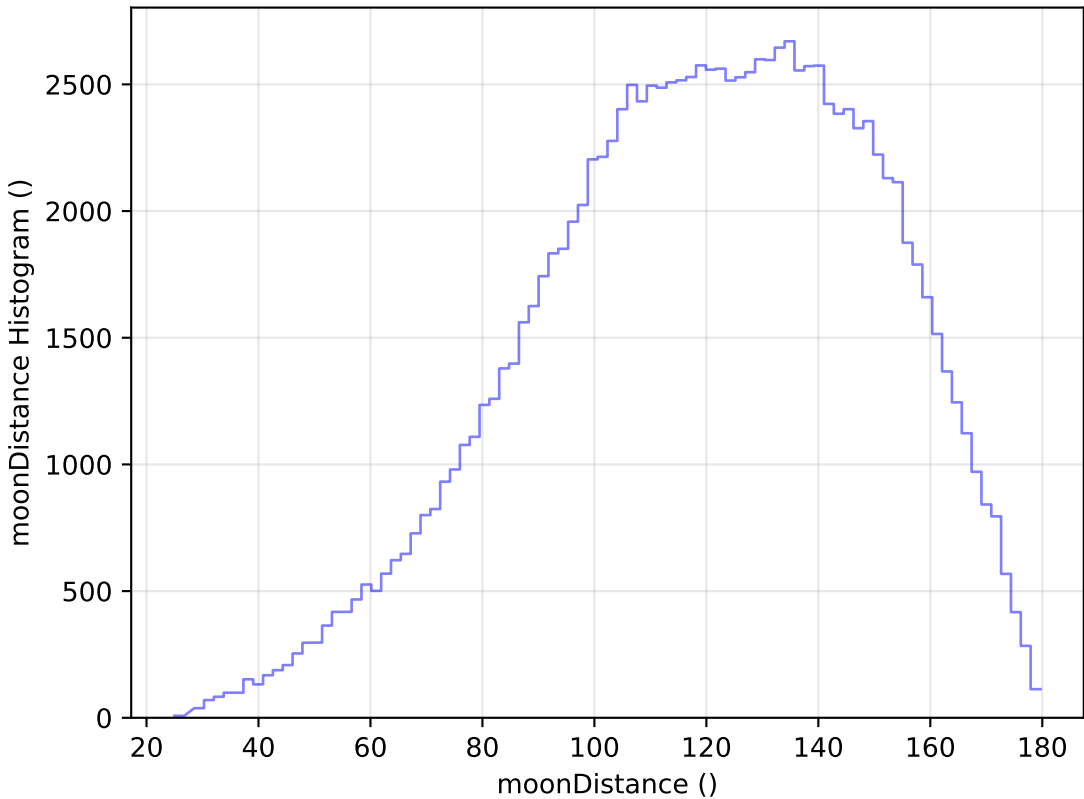
ddf_loaded_fl2_v3.4_10yrs All sky u band: moonDistance Histogram
