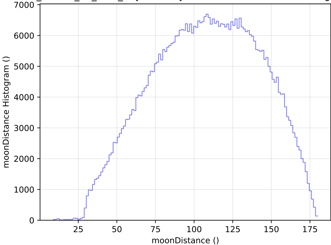
ddf_loaded_fl2_v3.4_10yrs All sky r band: moonDistance Histogram
