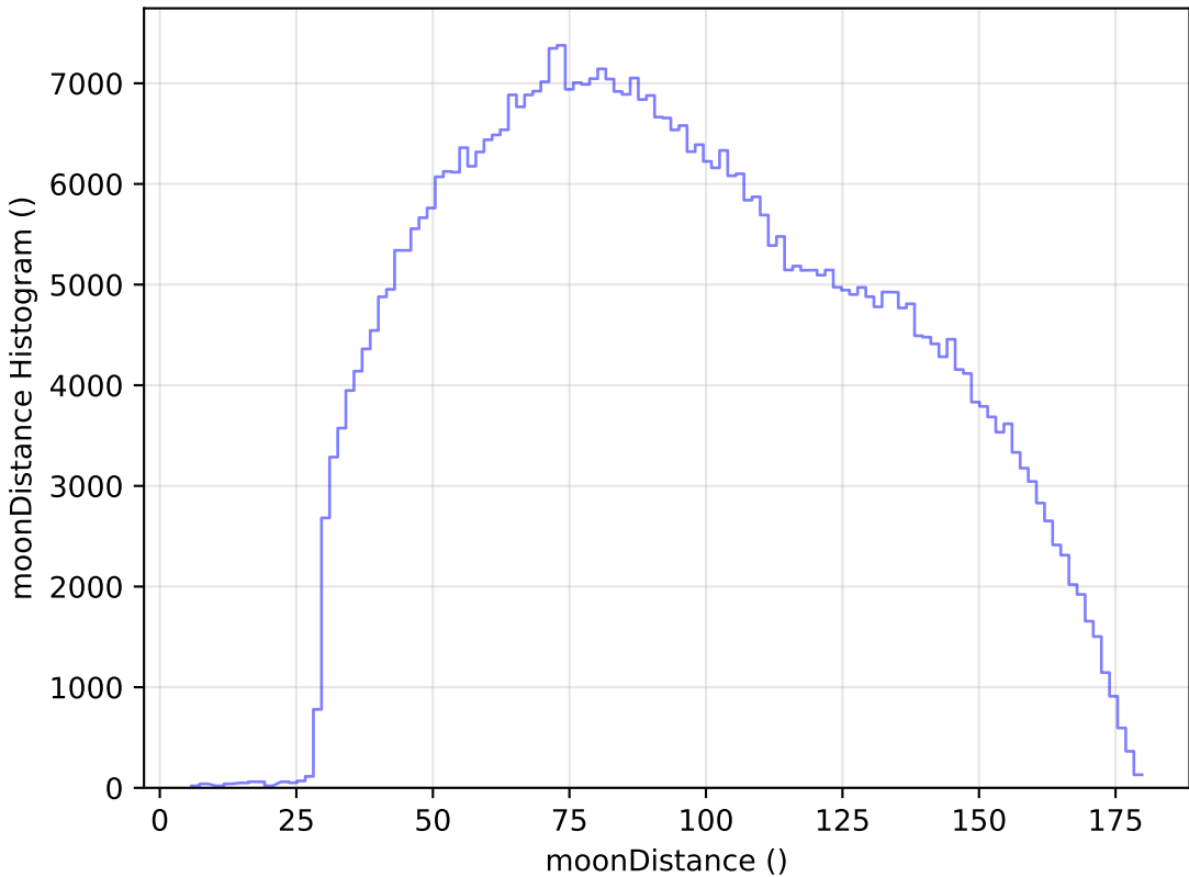
ddf_loaded_fl2_v3.4_10yrs All sky i band: moonDistance Histogram
