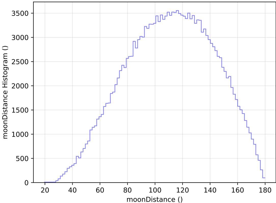
ddf_loaded_fl2_v3.4_10yrs All sky g band: moonDistance Histogram
