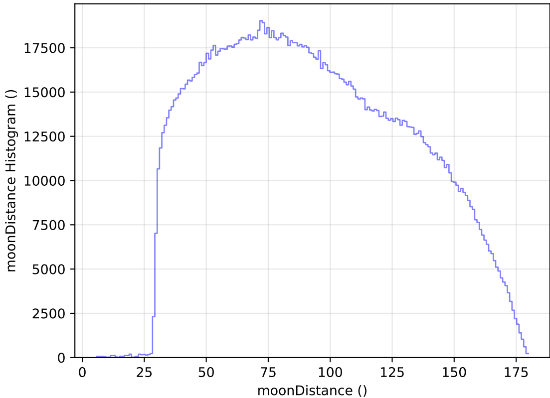
ddf_loaded_fl2_v3.4_10yrs All sky all bands: moonDistance Histogram
