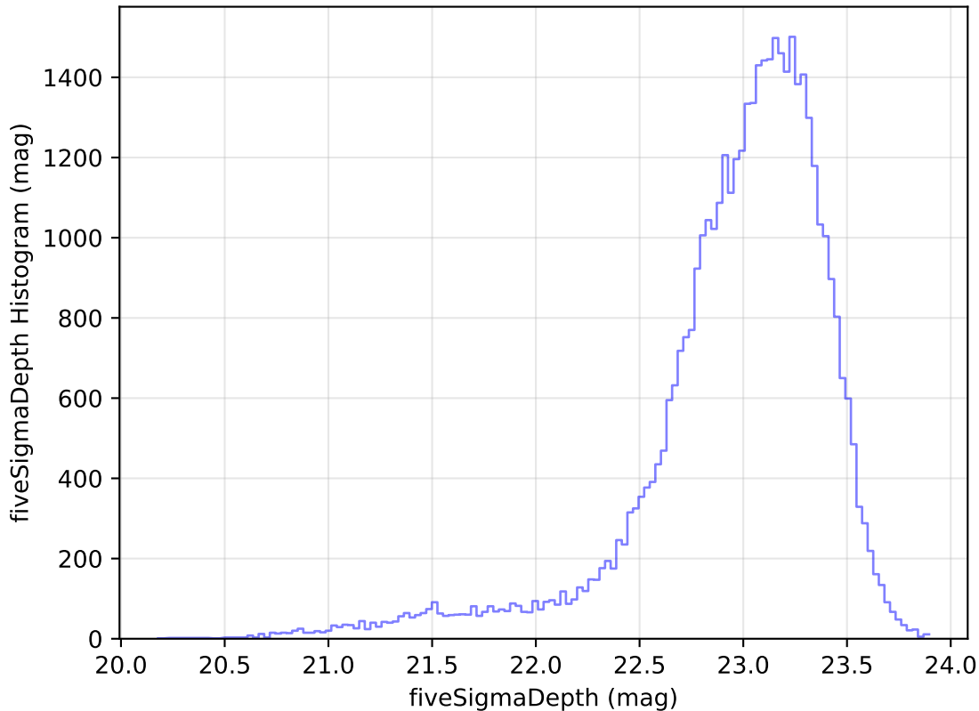
ddf_loaded_fl2_v3.4_10yrs Yr 1 z band: fiveSigmaDepth Histogram
