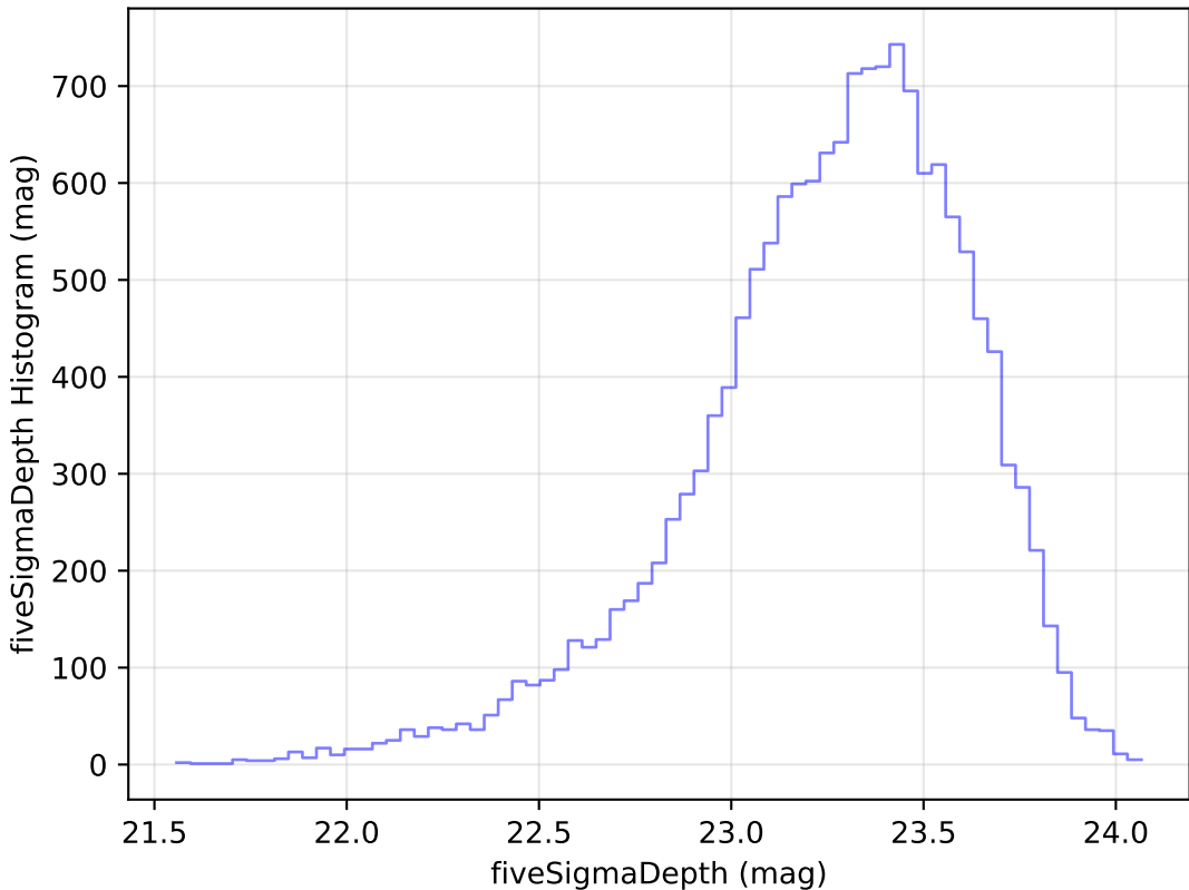
ddf_loaded_fl2_v3.4_10yrs Yr 1 u band: fiveSigmaDepth Histogram
