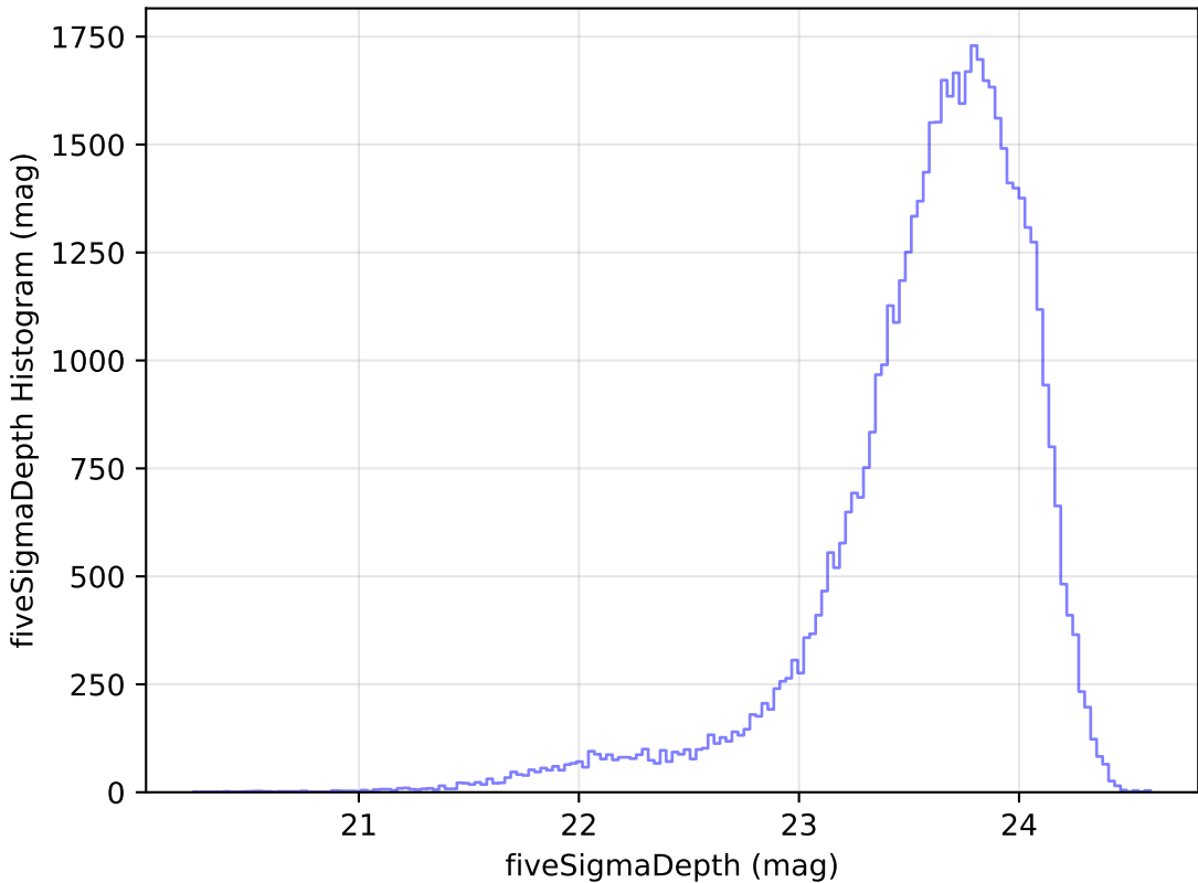
ddf_loaded_fl2_v3.4_10yrs Yr 1 i band: fiveSigmaDepth Histogram
