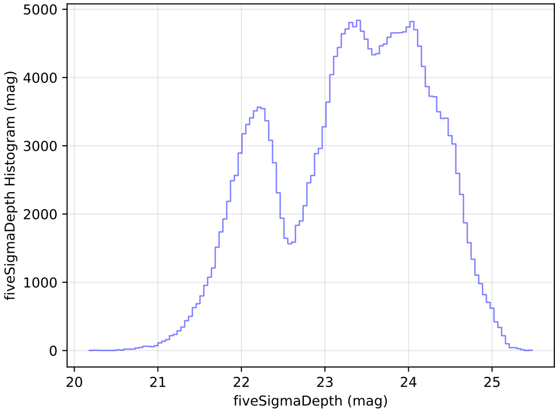
ddf_loaded_fl2_v3.4_10yrs Yr 1 all bands: fiveSigmaDepth Histogram
