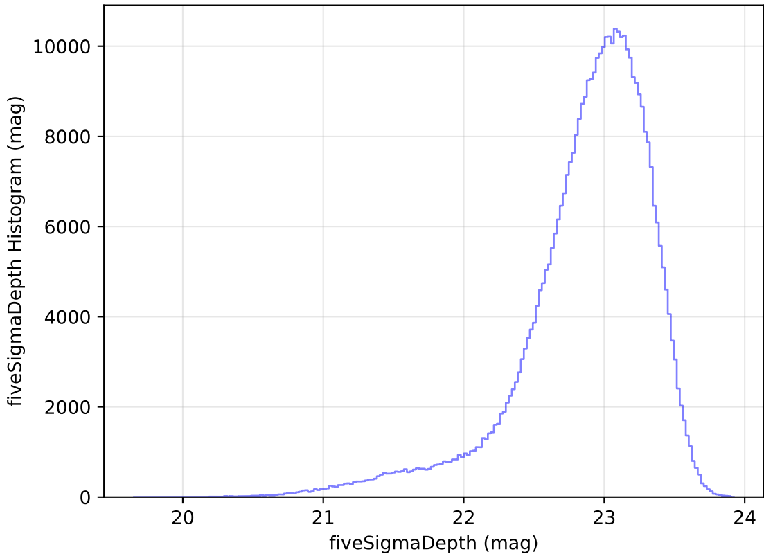
ddf_loaded_fl2_v3.4_10yrs WFD z band: fiveSigmaDepth Histogram
