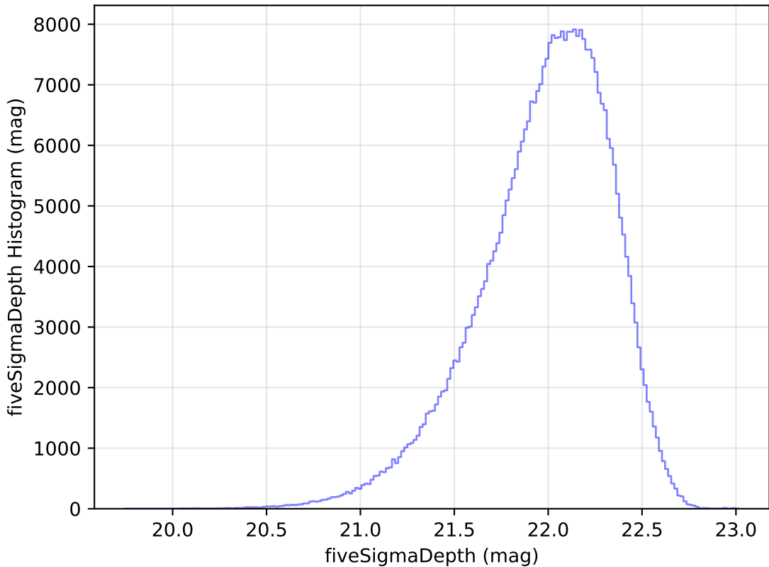
ddf_loaded_fl2_v3.4_10yrs WFD y band: fiveSigmaDepth Histogram
