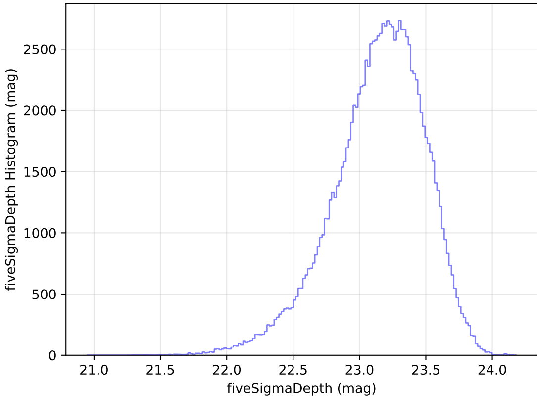
ddf_loaded_fl2_v3.4_10yrs WFD u band: fiveSigmaDepth Histogram
