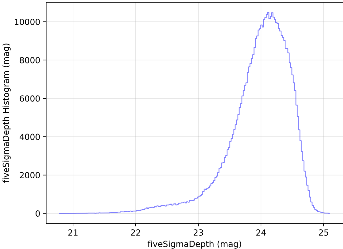
ddf_loaded_fl2_v3.4_10yrs WFD r band: fiveSigmaDepth Histogram
