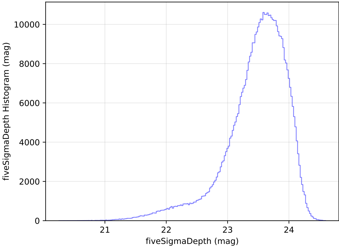
ddf_loaded_fl2_v3.4_10yrs WFD i band: fiveSigmaDepth Histogram
