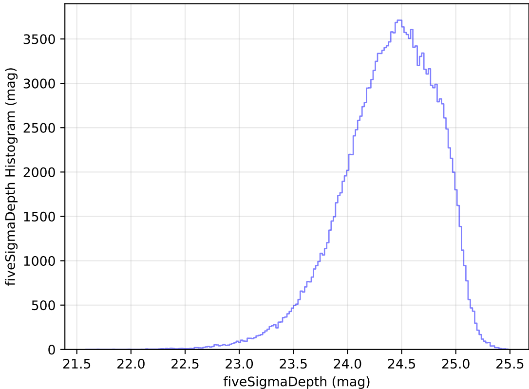
ddf_loaded_fl2_v3.4_10yrs WFD g band: fiveSigmaDepth Histogram
