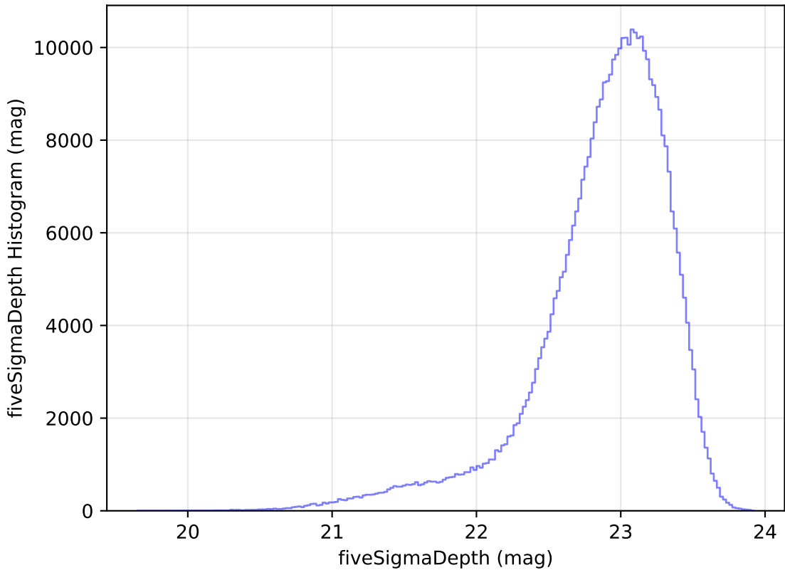
ddf_loaded_fl2_v3.4_10yrs All sky z band: fiveSigmaDepth Histogram
