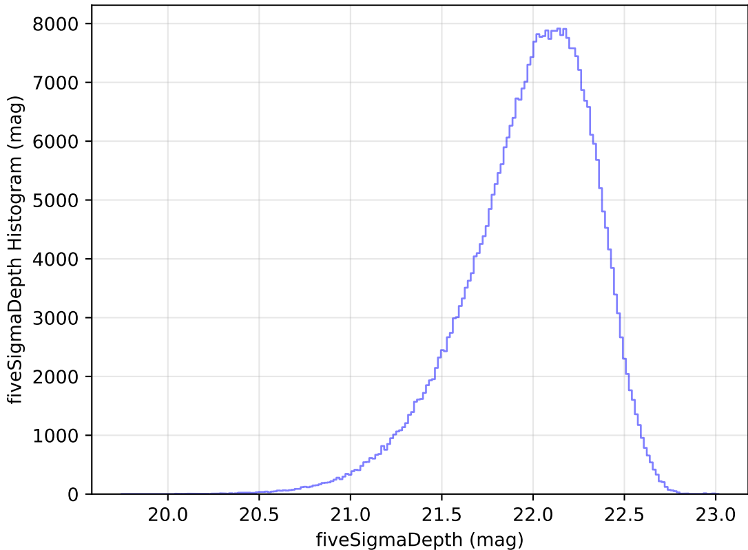
ddf_loaded_fl2_v3.4_10yrs All sky y band: fiveSigmaDepth Histogram
