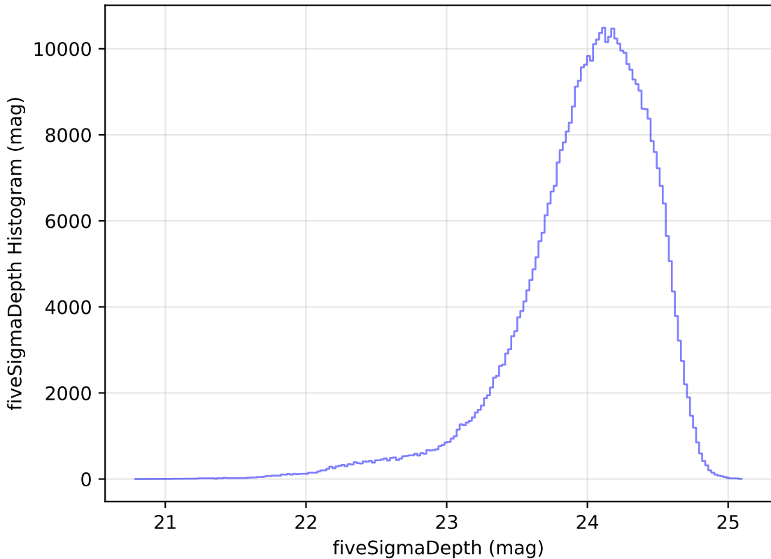
ddf_loaded_fl2_v3.4_10yrs All sky r band: fiveSigmaDepth Histogram
