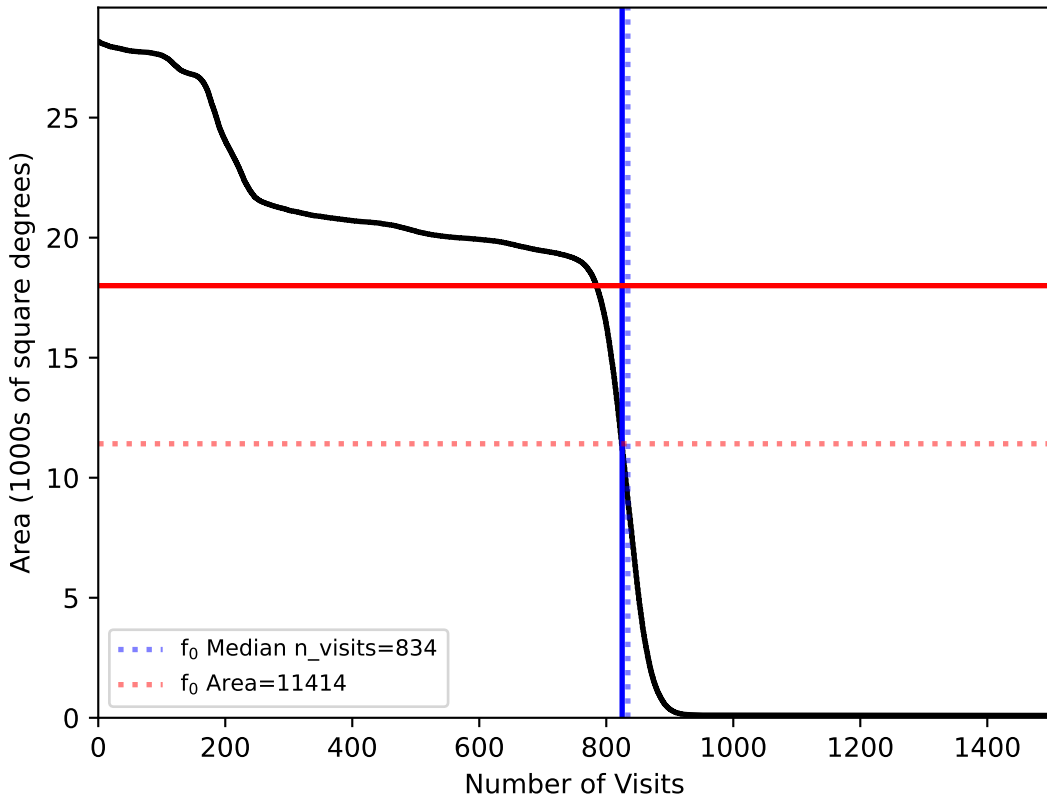
ddf_loaded_fl2_v3.4_10yrs All sky: f0
