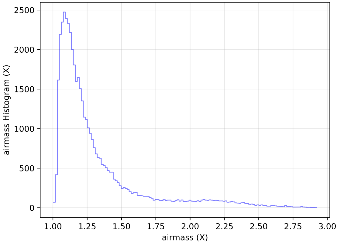
ddf_loaded_fl2_v3.4_10yrs Yr 1 z band: airmass Histogram
