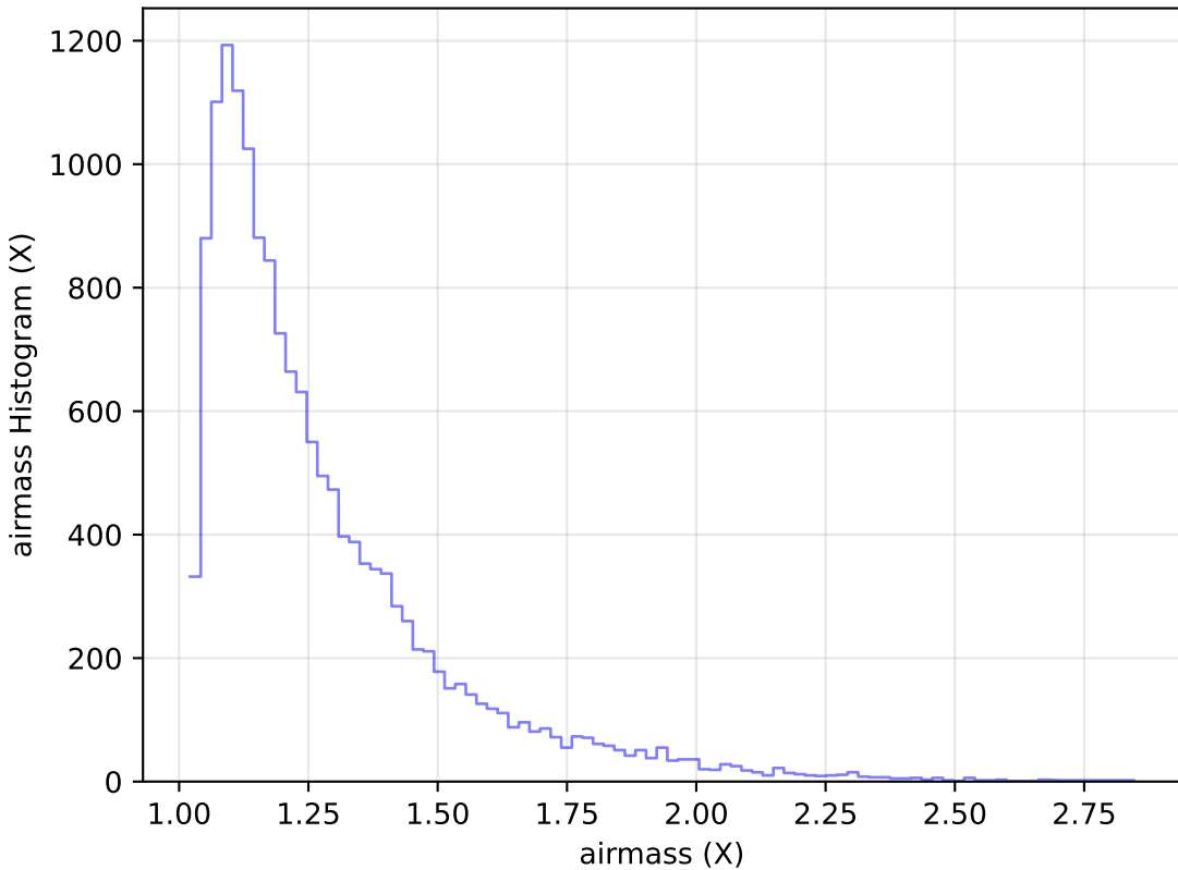
ddf_loaded_fl2_v3.4_10yrs Yr 1 u band: airmass Histogram
