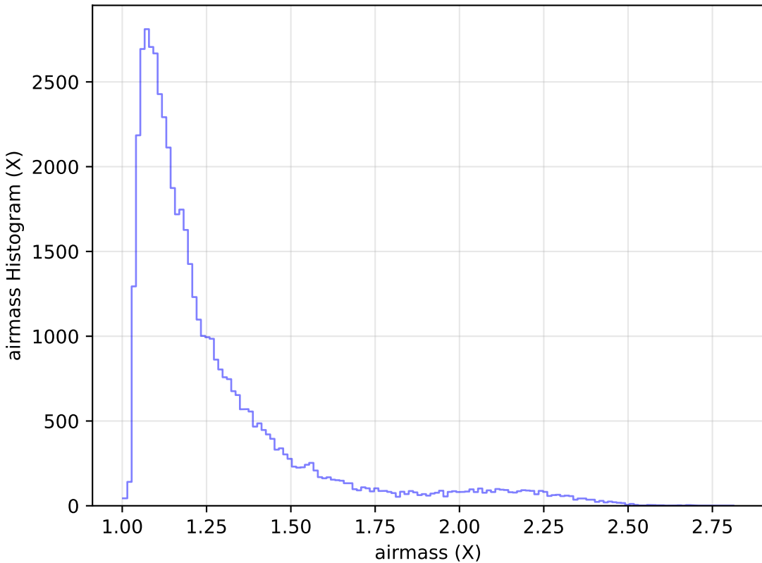
ddf_loaded_fl2_v3.4_10yrs Yr 1 r band: airmass Histogram
