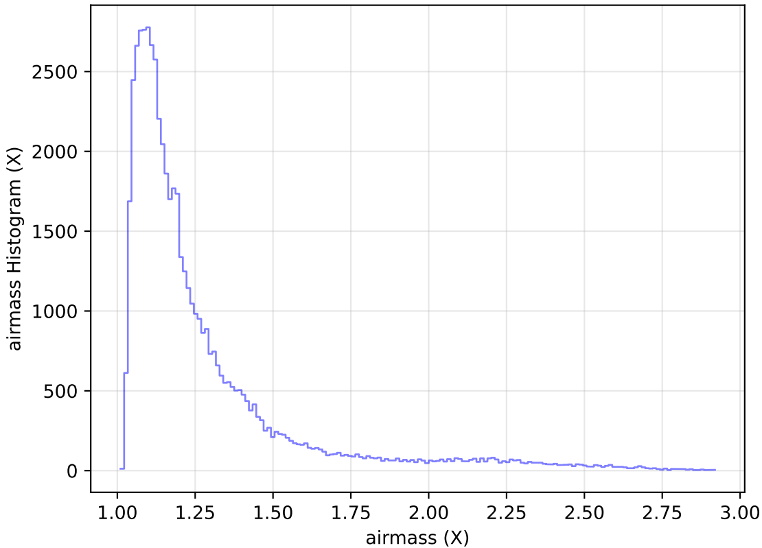
ddf_loaded_fl2_v3.4_10yrs Yr 1 i band: airmass Histogram
